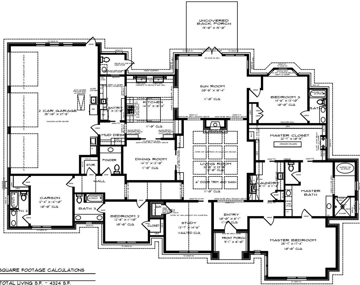
FLOOR PLAN
