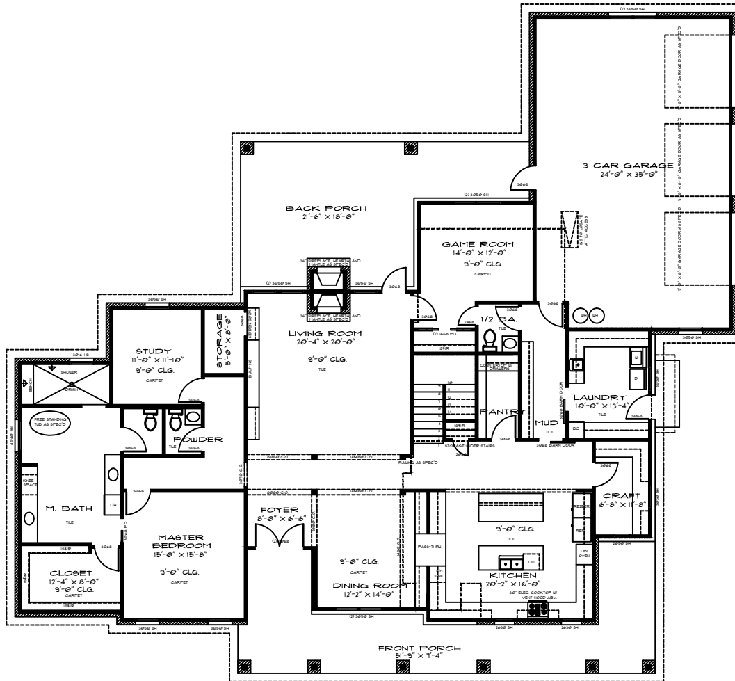
FLOOR PLAN
