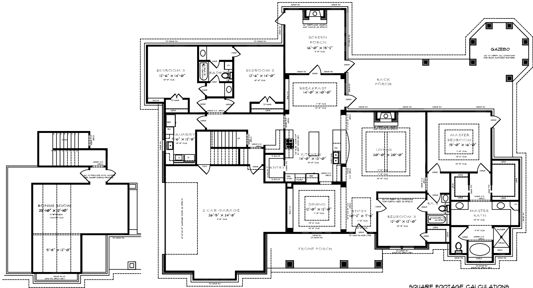
BONUS FLOOR PLAN
