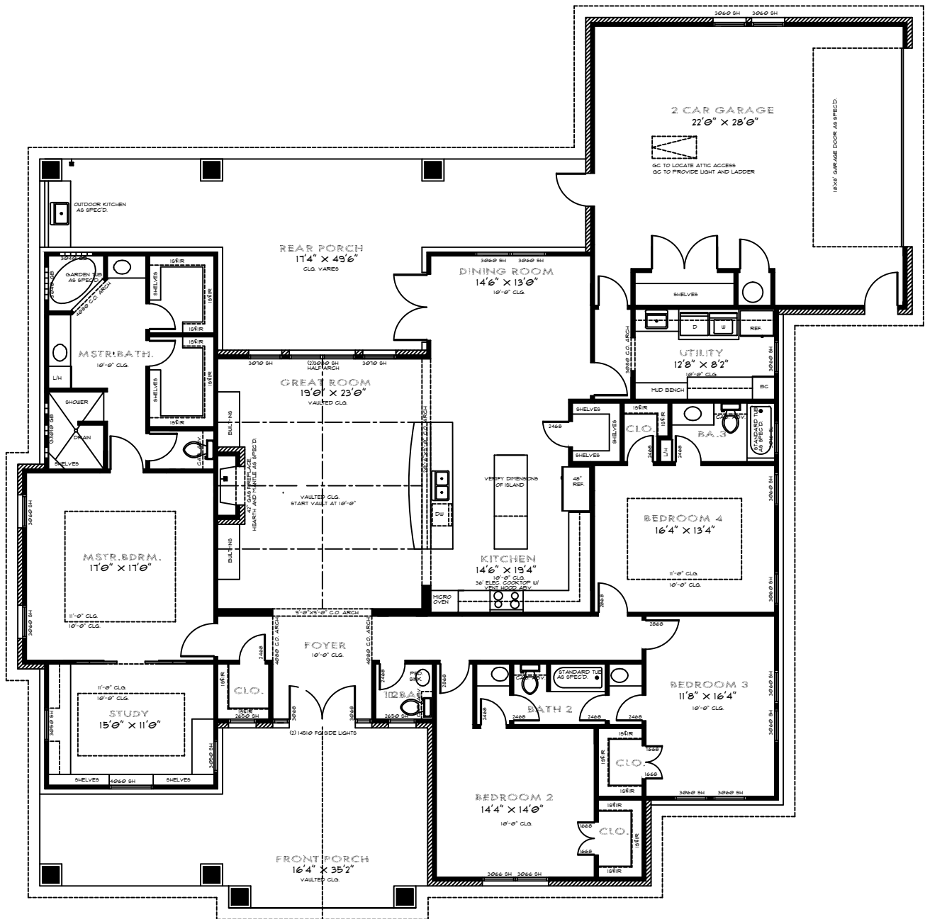
FLOOR PLAN
