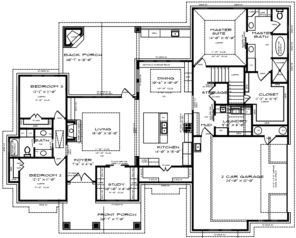
FLOOR PLAN
