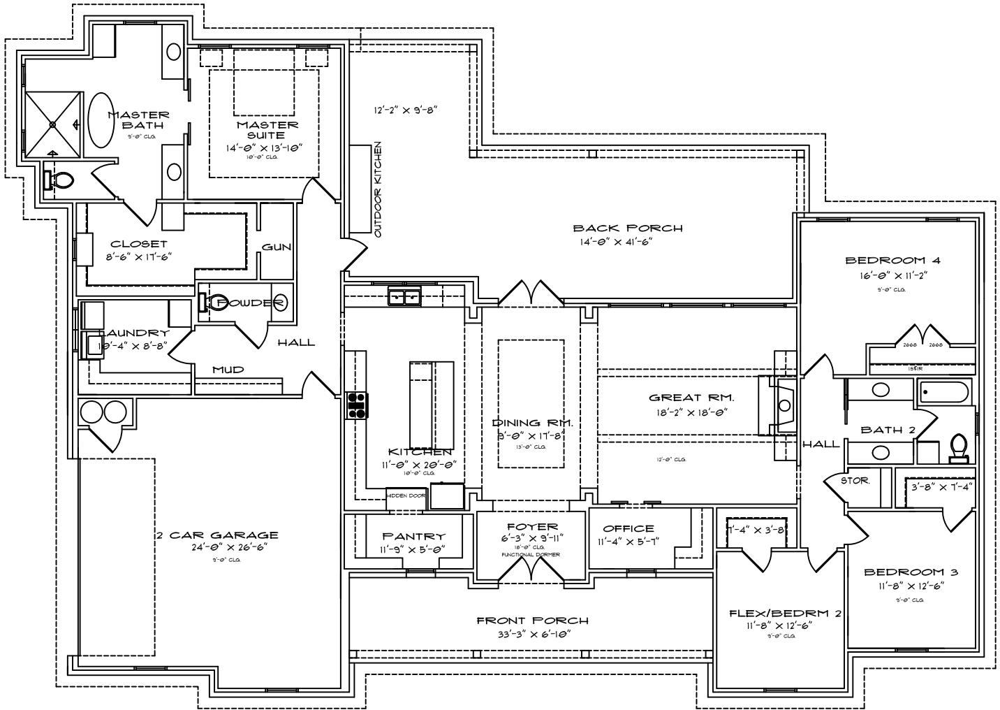
FLOOR PLAN
