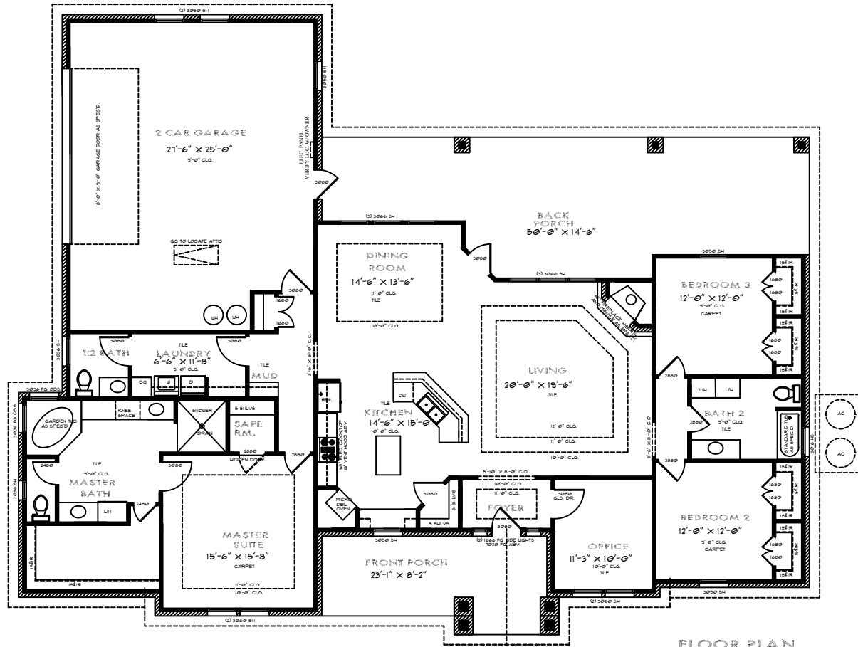
FLOOR PLAN
