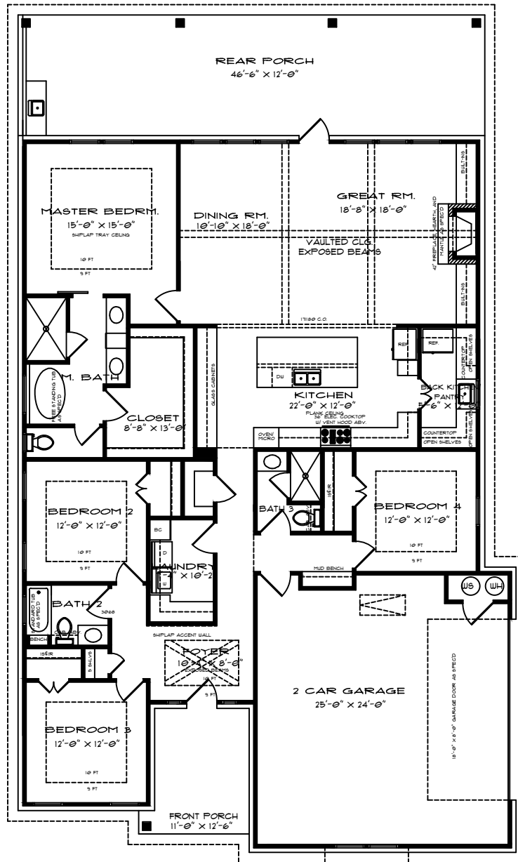
FLOOR PLAN
