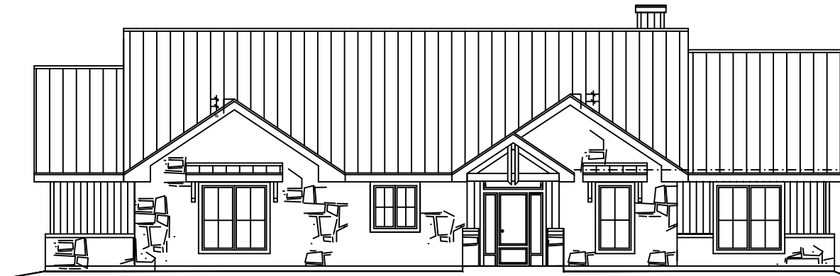
FRONT ELEVATION
