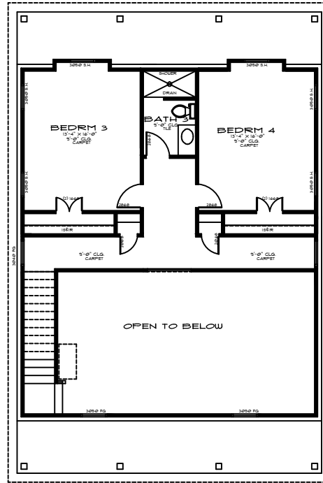
2ND LEVEL FLOOR PLAN
