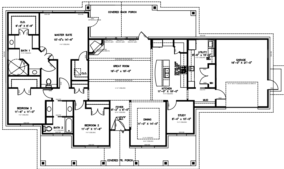
FLOOR PLAN NOT TO SCALE
