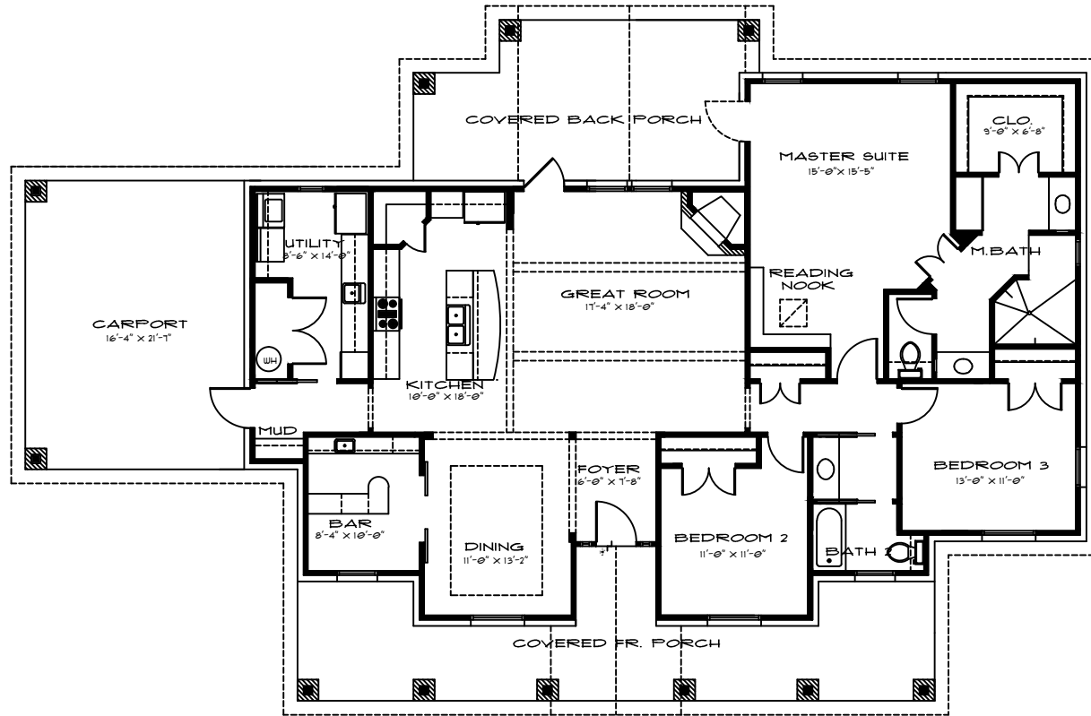
FLOOR PLAN
