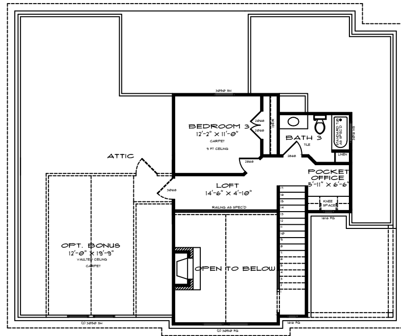
2ND LEVEL FLOOR PLAN
