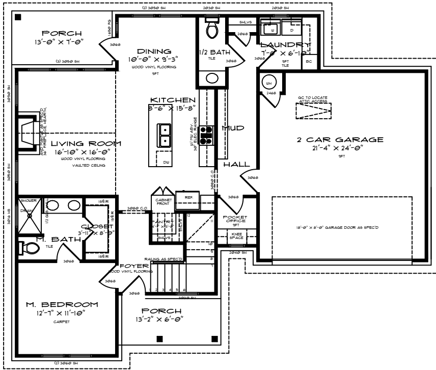
MAIN LEVEL FLOOR PLAN
