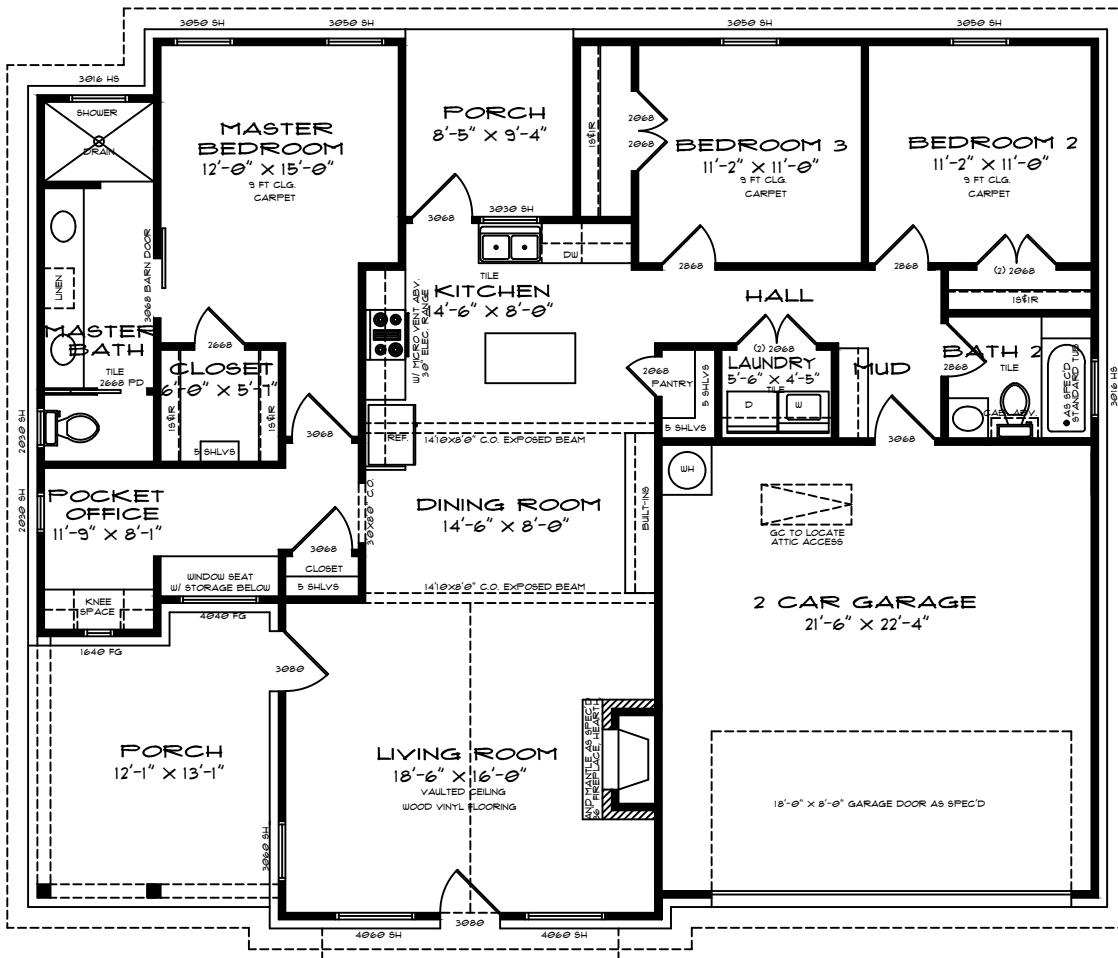
FLOOR PLAN
