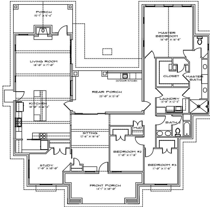
FLOOR PLAN
