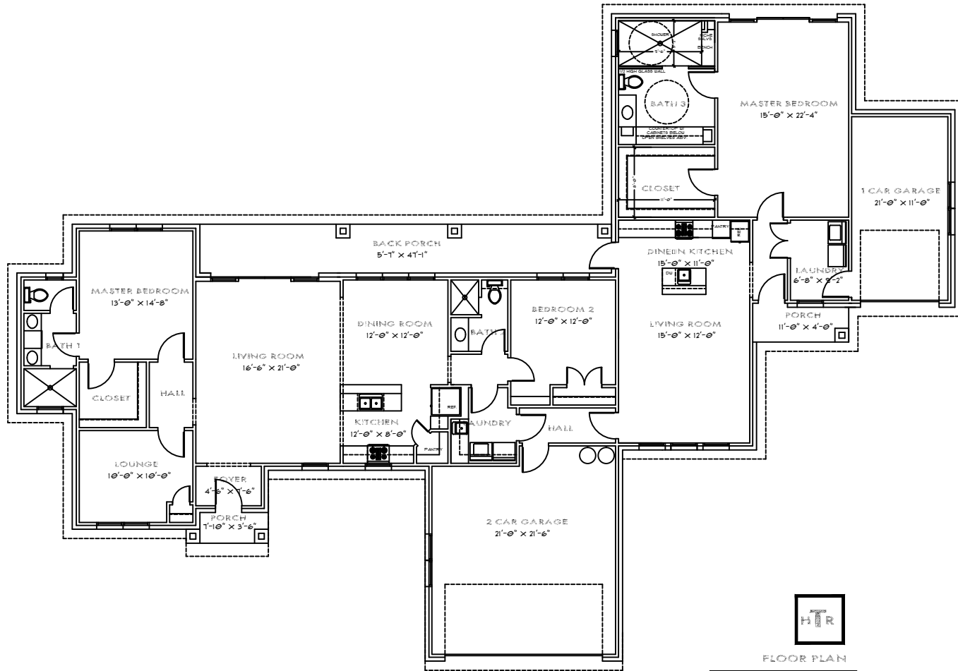
FLOOR PLAN
