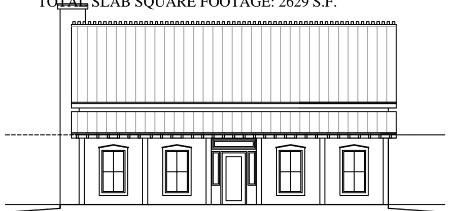
FRONT ELEVATION NOT TO SCALE
