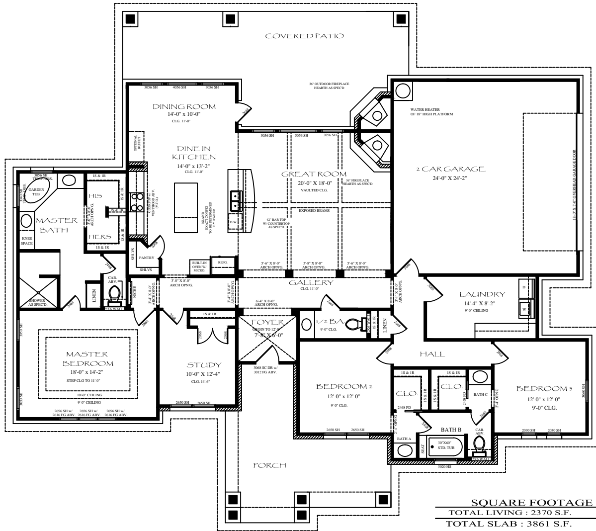
FLOOR PLAN
