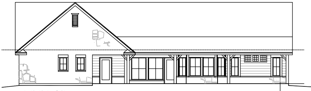
BACK ELEVATION
