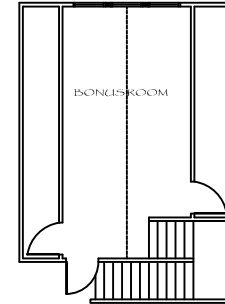
BONUS ROOM FLOOR PLAN SCALE: 1/4" = 1'-0"
